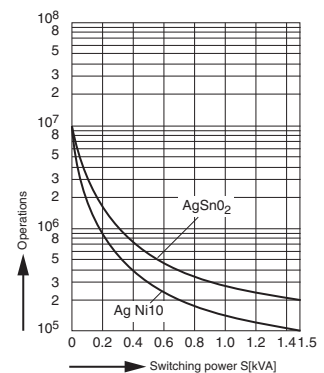
Mechanical life
